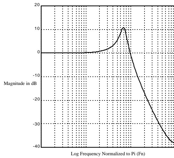
Figure 6: Filter Resonance
