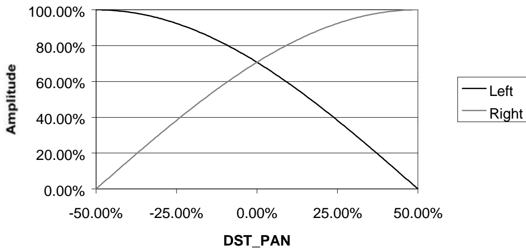
Figure 11: Pan Curve
